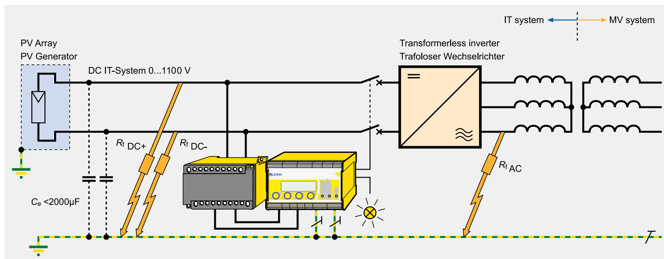
PV generator unearthed (IT system) with nominal voltage \leq 1100\text{ V} and ISOMETER® isoPV with coupling device AGH-PV
